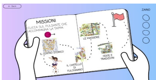
Escape-game
